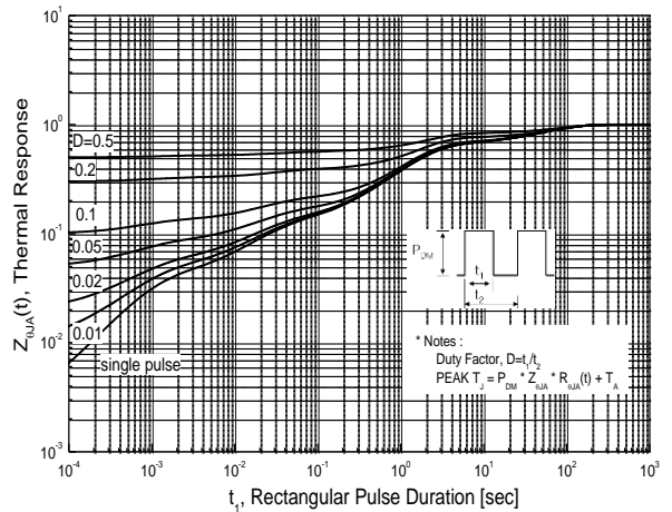
Fig.12 Transient Thermal Response Curve (Junction-to-Ambient)
