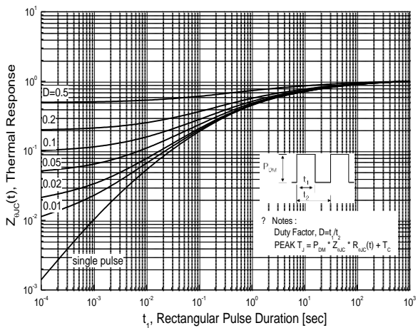
Fig.11 Transient Thermal Response Curve (Junction-to-Case)
