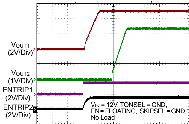
VOUT2 Delay-Start
