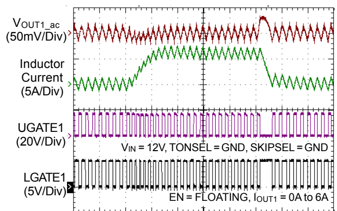
VOUT1 PWM-Mode Load Transient Response
