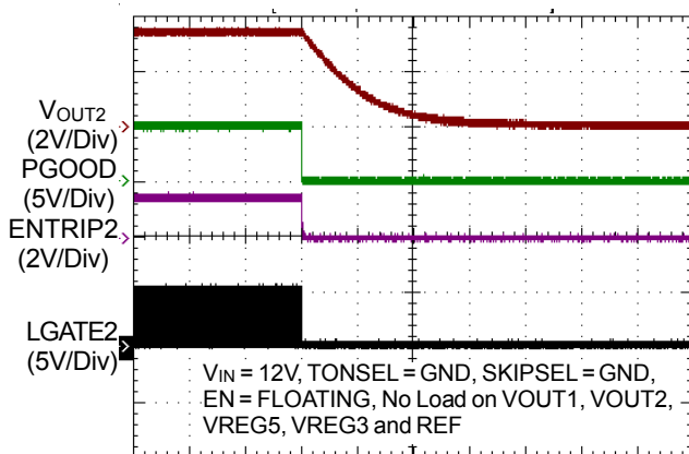
Power Off from ENTRIP2
