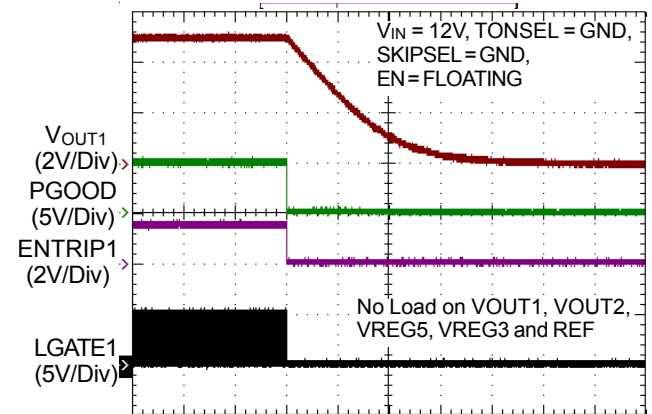
Power Off from ENTRIP1
