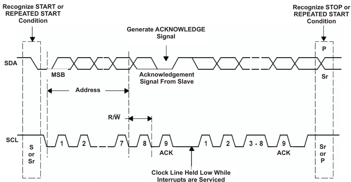
Figure 33. Bus Protocol
