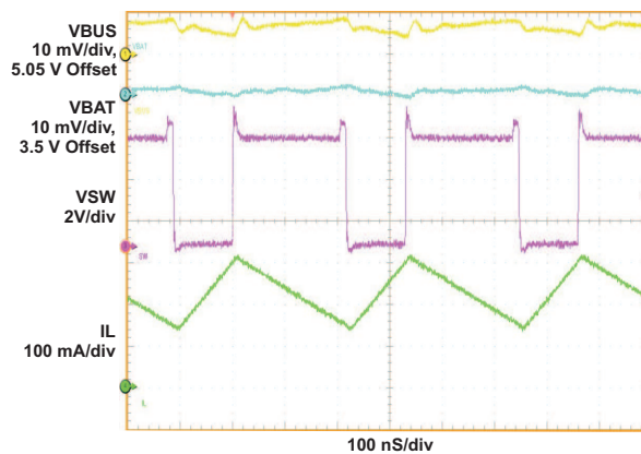
Figure 14. VBUS = 5.05 V, VBAT = 3.5V, I BUS = 217 mA
